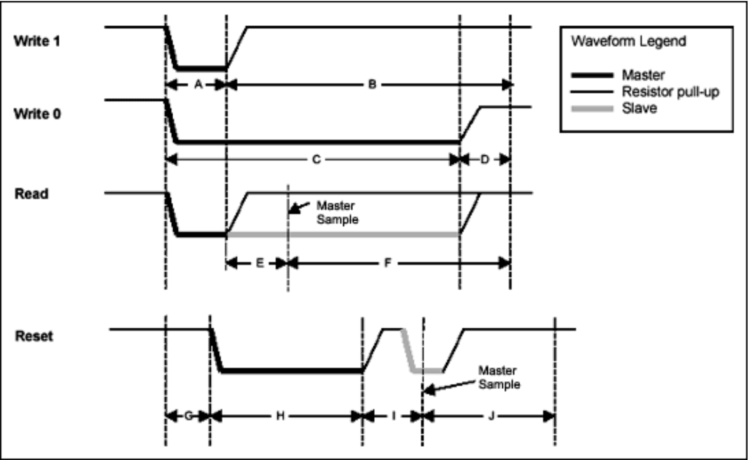
Figure 1. 1-Wire waveforms.
